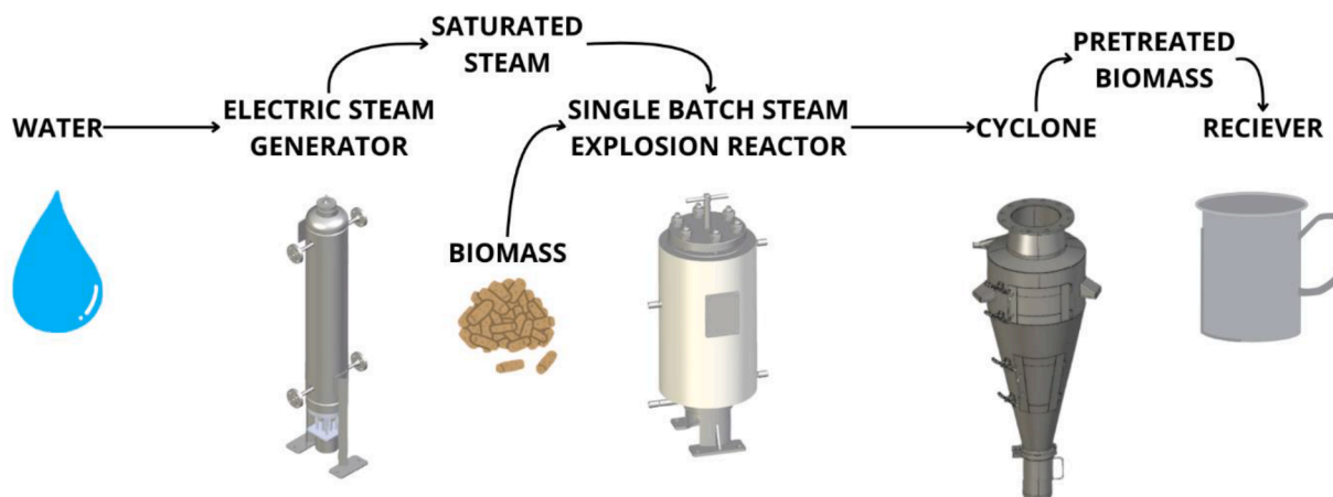
Fig. 1. Simplified scheme of steam explosion process.
