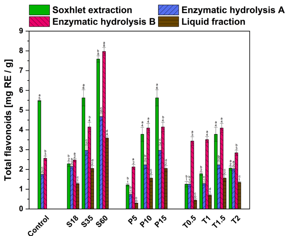
Fig. 7. Effects of SE, pressure, duration and particle size on total flavonoid content in the TSRs, expressed in mg RE per g of biomass. Pretreatment conditions comprised 3 modes - sieve (S), pressure (P) and time (T). As a control, the untreated sample S35 was considered. Different letters within each experimental group (Sn, Pn, Tn) indicate statistically significant differences (Tukey HSD, P < 0.05 ).
