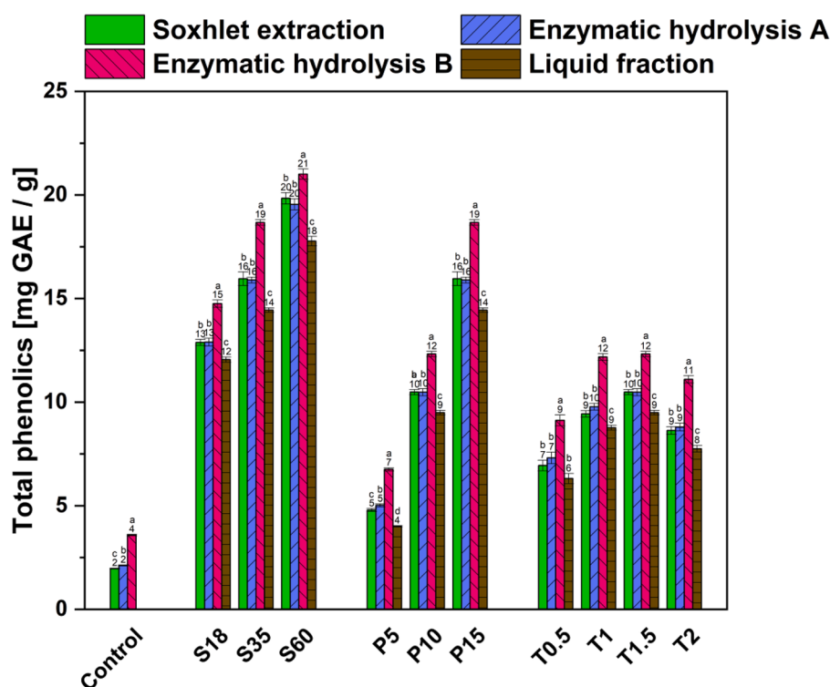
Fig. 6. Effects of three SE factors (pressure, duration and particle size) on total phenolic content in the TSRs, expressed in mg GAE per g of biomass, quantified by UV–Vis spectrophotometry. Pretreatment conditions comprised 3 modes - sieve (S), pressure (P) and time (T). As a control, the untreated sample S35 was considered. Different letters within each experimental group (Sn, Pn, Tn) indicate statistically significant differences (Tukey HSD, P < 0.05 ).
