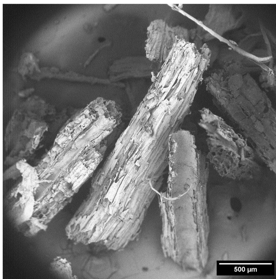
Fig. 4. Structural overview of the untreated TSR S30 sample at 150x magnification.
