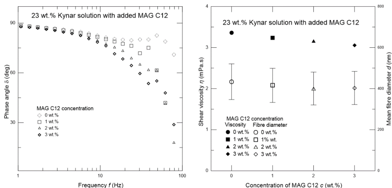
Figure 2 Phase angle (left), shear viscosity of polymer solutions (right) and mean fibre diameter of electrospun nanofibres (right)
