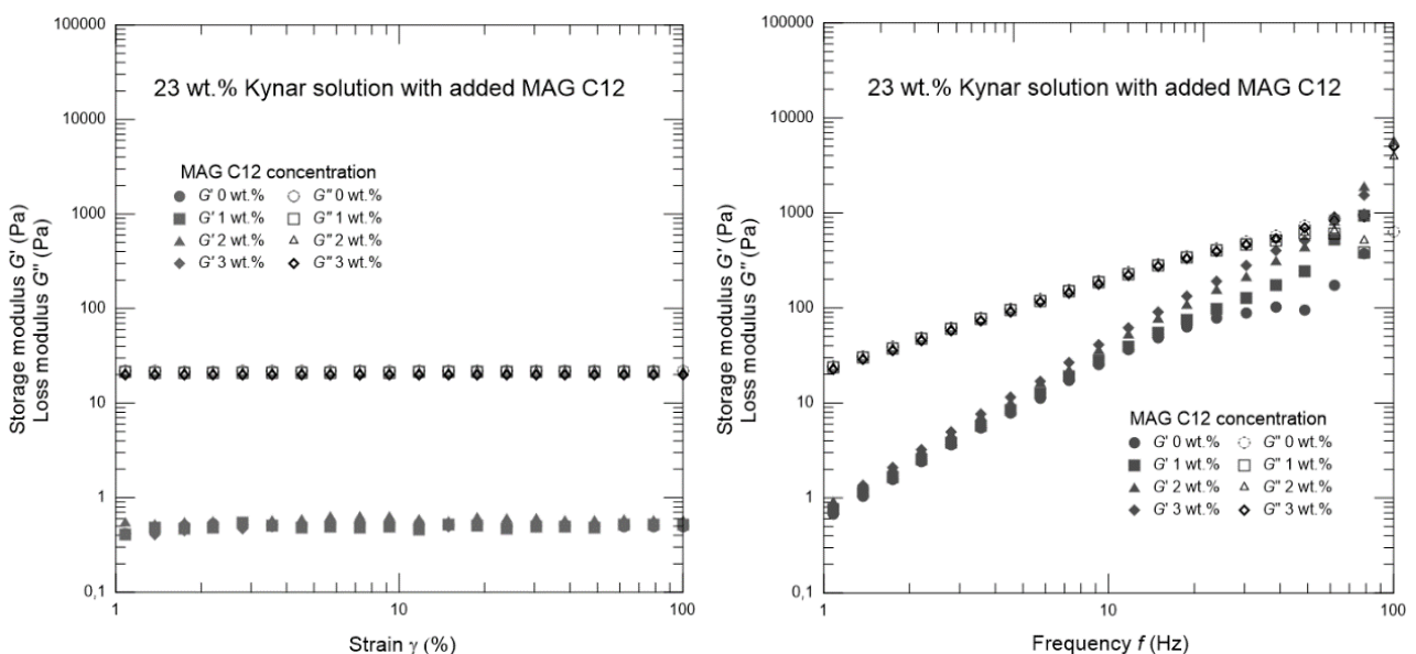
Figure 1 Oscillatory strain (left) and frequency (right) sweep measurements characterizing viscoelastic nature of polymer solutions
