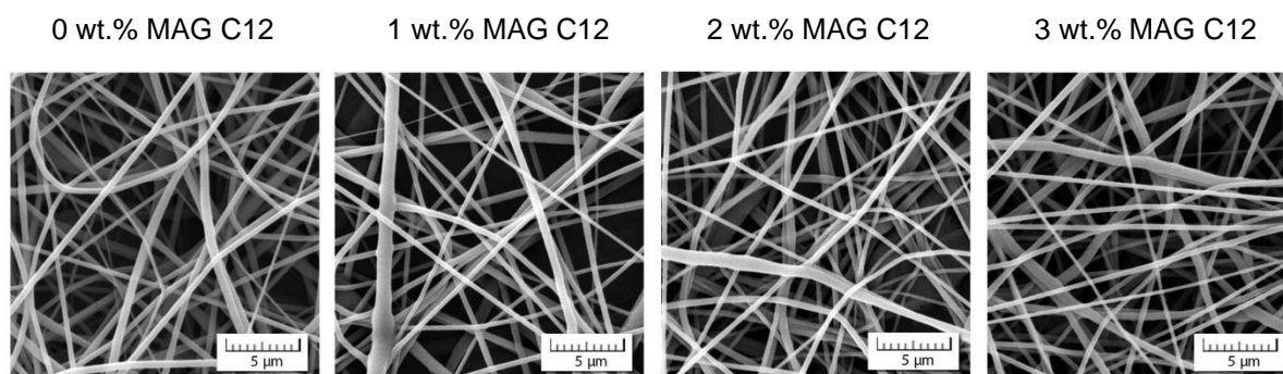
Figure 3 The quality of nanofibrous mats without/with added MAG C12
