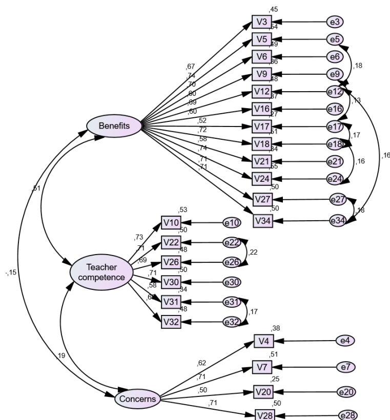
Figure 1. Path diagram of the confirmatory factor analysis of DPBA.
