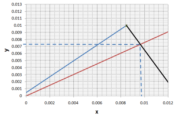
Fig. 2: Operation line (blue), equilibrium line (red) and interface composition ( P_1 M_1 ) (dashed line).
