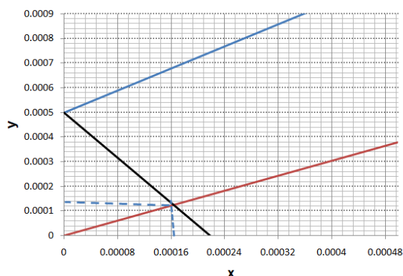
Fig. 3: Operation line (blue), equilibrium line (red) and interface composition ( P_2M_2 ) (dashed line).
