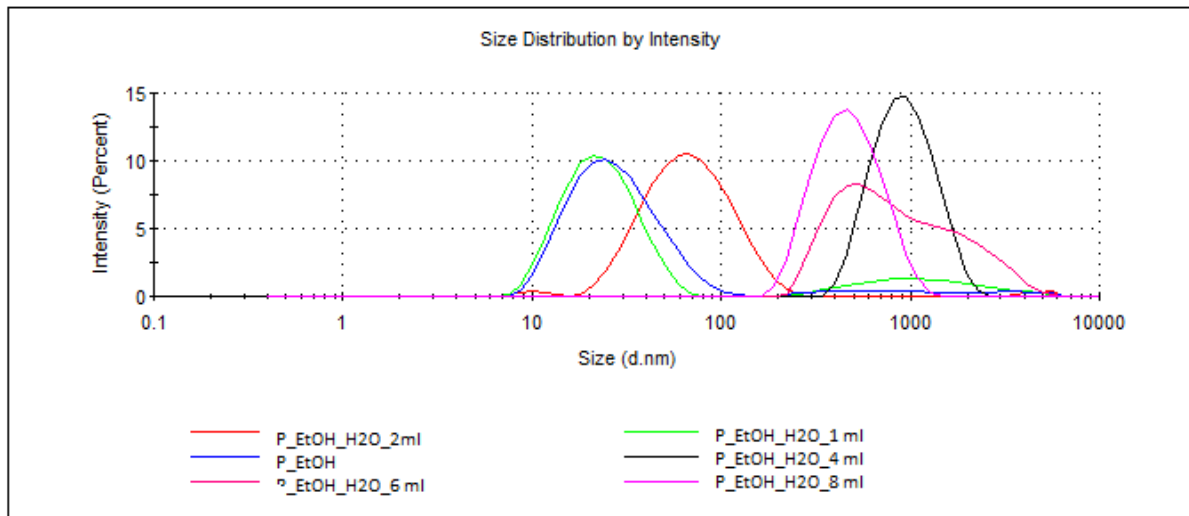
Fig. 2 - DLS size distribution curves of Paraloid B72 dispersion in EtOH with water additions.
