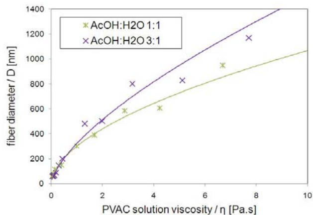
FIGURE 5. Dependence of fiber diameter ( D ) on PVAC solution viscosity ( \eta ) in solvent system AA : H 2 O – 3:1 (v/v) and AA : H 2 O – 1:1 (v/v).
