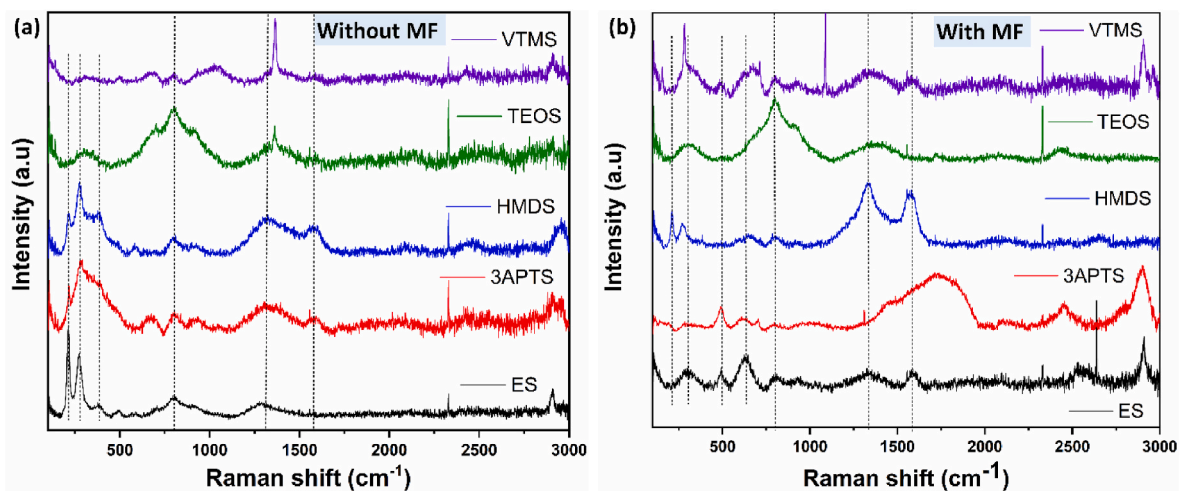
Fig. 17. Raman spectroscopy of worn-out surface for bare CIPs and organosilane coated CIPs based MRF (a) without magnetic field, (b) with magnetic field.
