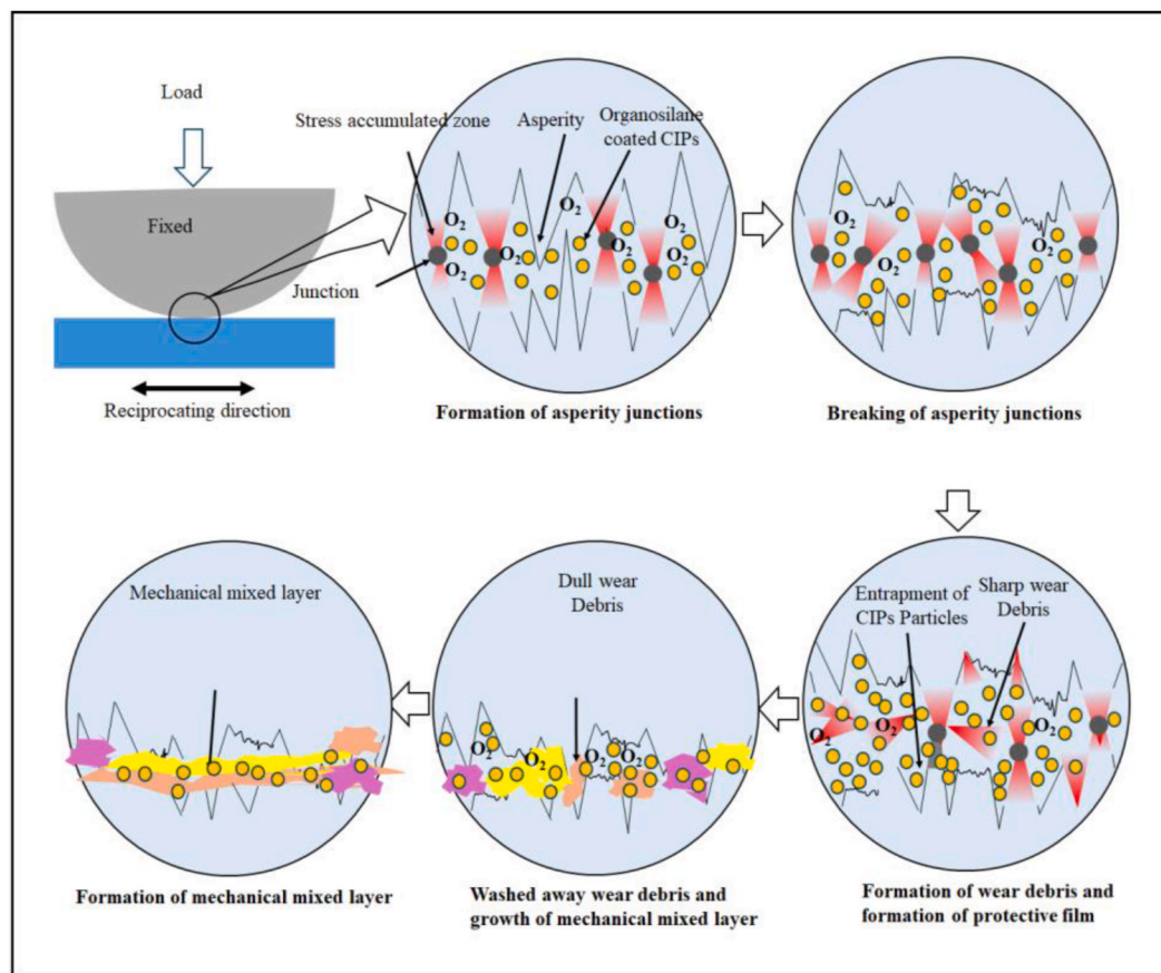
Fig. 16. Schematic of the formation of the mechanically mixed layer at the contact interface under MRF lubricating sliding condition.
