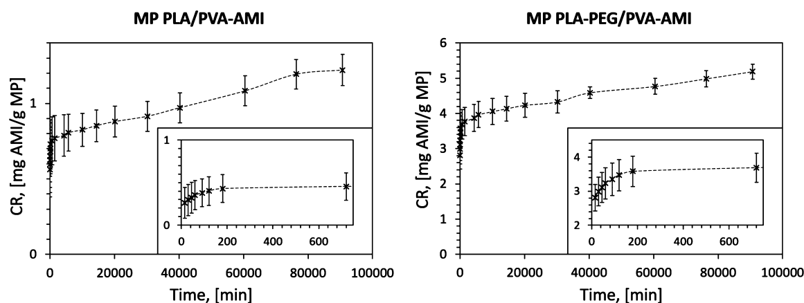
Figure 8. AMI release from MP PLA/PVA and MP PLA-PEG/PVA (SD—three independently prepared material samples).
