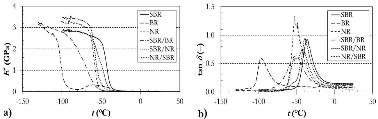
Fig. 1 Temperature dependencies of the tensile storage modulus (a) and the loss factor (b) of the tested rubber samples at the sample deformation x = 5 \mu m and the frequency f = 1 \text{ Hz}
