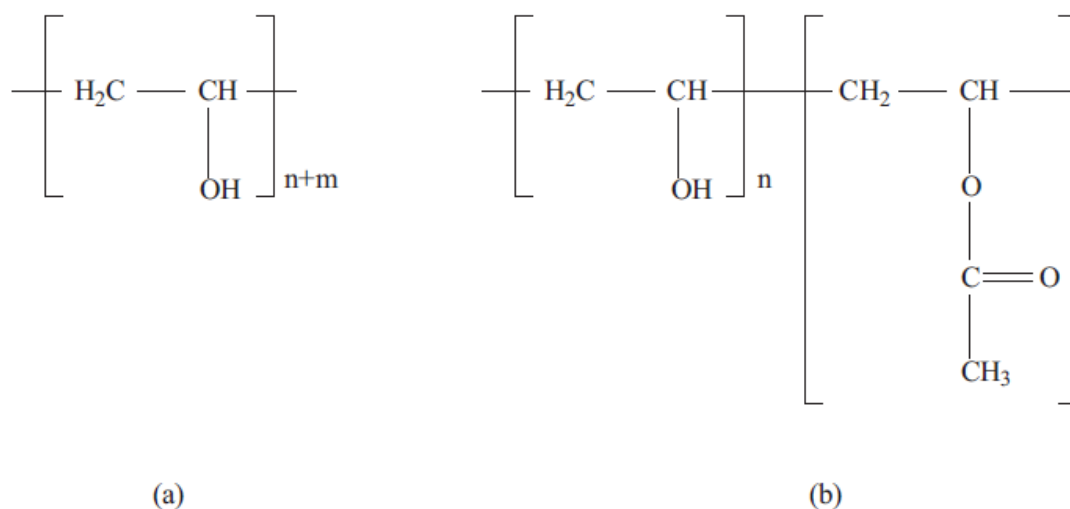
Fig. 1. Molecular structure of fully hydrolyzed (a) and partially hydrolyzed (b) PVA.
