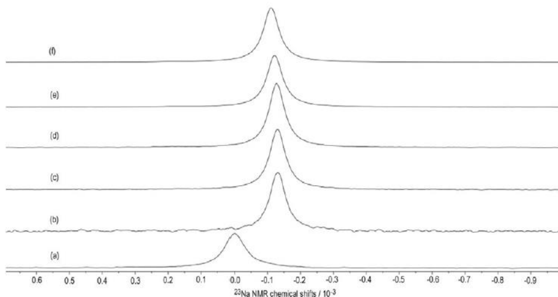
Fig. 3. 23 Na NMR spectra of a D 2 O solution of PVA 0.0089 mol kg -1 , at 25 °C as a function of increasing concentrations of NaCl: (a) 0.0089 mol kg -1 alone (external reference) and (b) 0.0045 mol kg -1 ; (c) 0.0089 mol kg -1 ; (d) 0.0178 mol kg -1 ; (e) 0.0445 mol kg -1 and (f) 0.0890 mol kg -1 .
