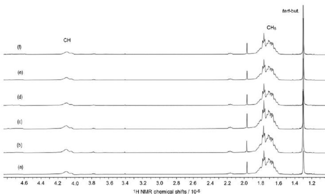
Fig. 4. 1 H NMR spectra of a D 2 O solution of PVA 0.0089 mol kg -1 at 25 °C as a function of increasing concentrations of NaCl: (a) 0, pH* 6.77, (b) 0.0045 mol kg -1 (c) 0.0089 mol kg -1 (d) 0.0178 mol kg -1 , (e) 0.0445 mol kg -1 and (f) 0.0890 mol kg -1 .
