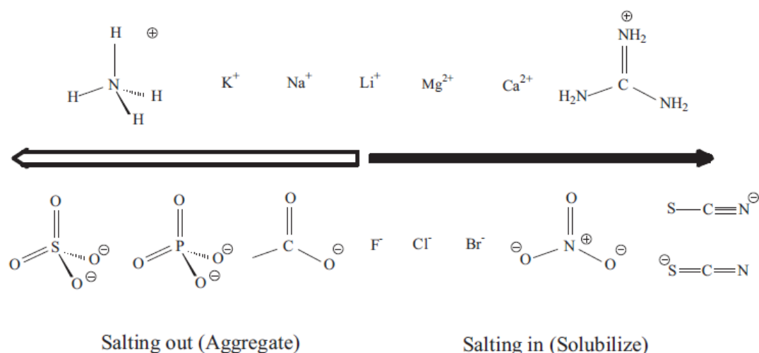
Fig. 2. Typical ordering of Hofmeister ions series based on precipitation studies of solutions of typical and anionic proteins [18,19].
