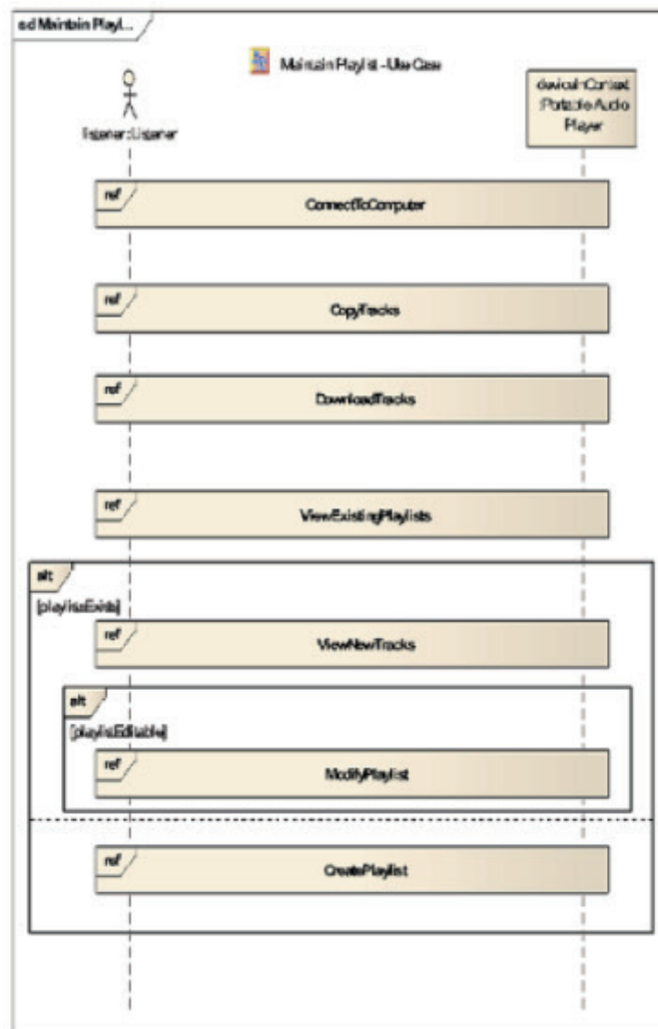
Fig. 3 Sequence Diagram for Playlist Maintaining
