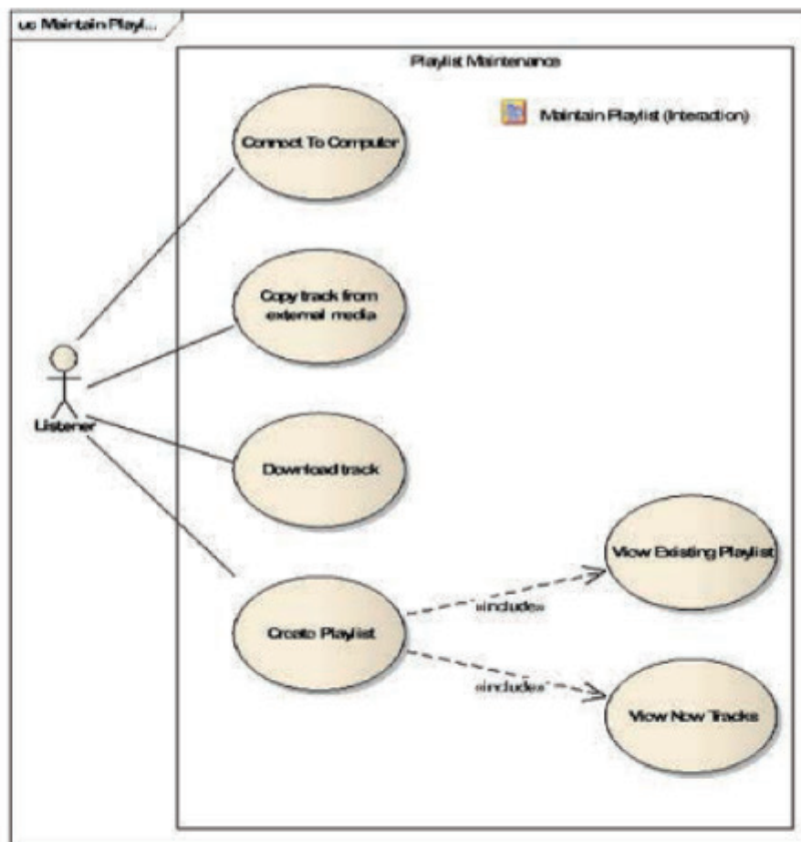
Fig. 2 Use Case Model
