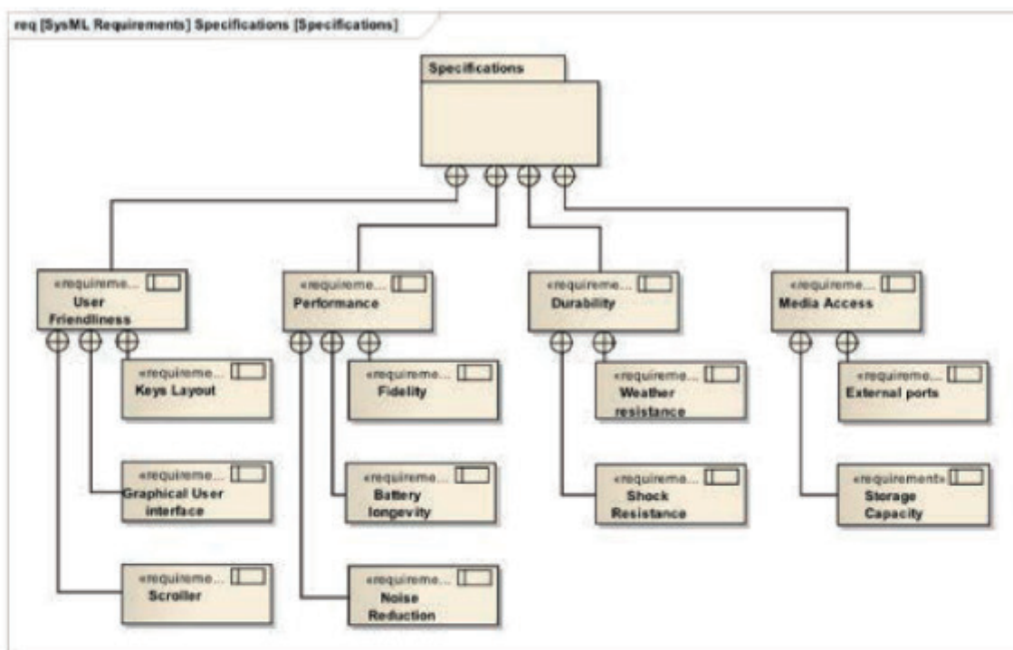
Fig. 1 Requirements Model
