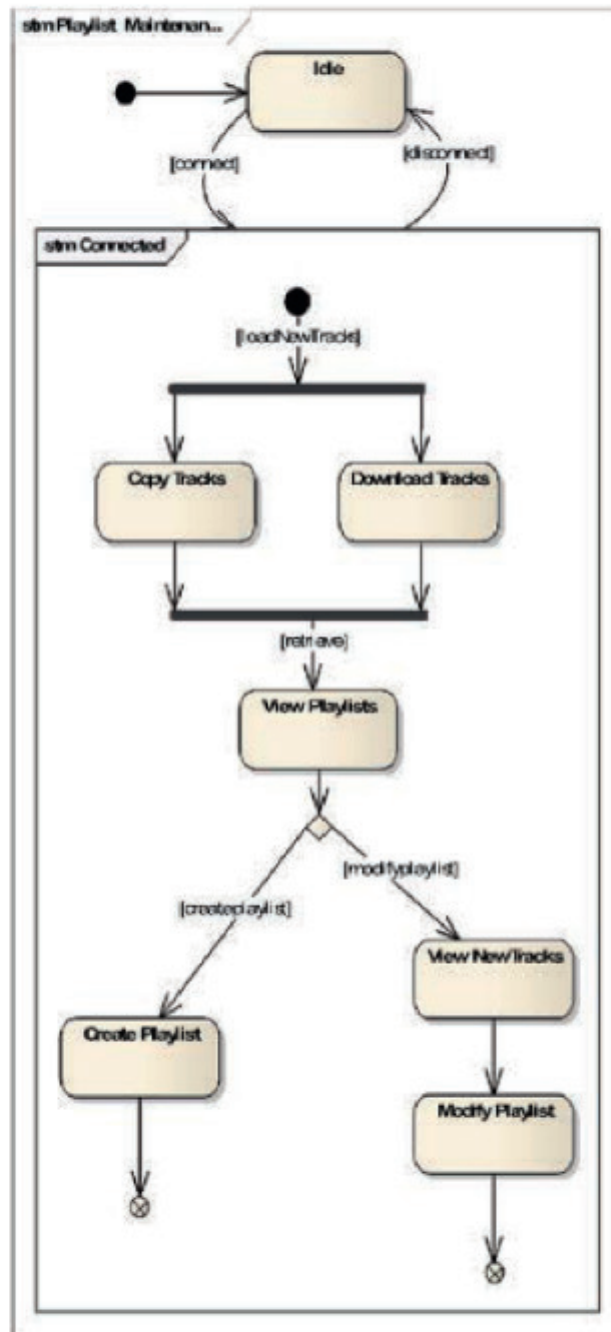
Fig. 4 State Machine Diagram with Activity
