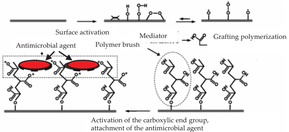
Figure 5. Schematic representation of antimicrobial agent immobilization on a polymer surface mediated by a polymer brush [43]
