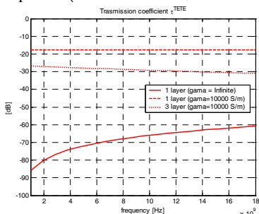
Fig. 14. Transmission coefficient of the composite structure (Number of Floquet harmonics M = N = 18 ), angle of incidence \nu^l = 0 \text{ deg} , \varphi^l = 90 \text{ deg} (electric intensity parallel with wire).
