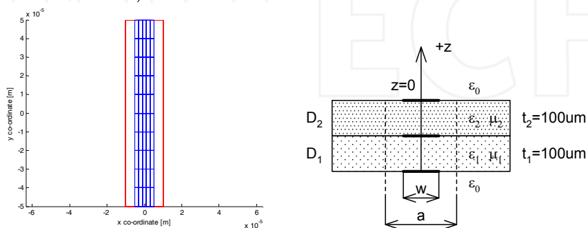
Fig. 13. Composite material with carbon fibres ( a = 20 \mu\text{m} , w = 10 \mu\text{m} , t = 10 \mu\text{m} ) Left) Meshed fibre, Right) Profile of the composite ( t_1 = t_2 = 100 \mu\text{m} , \epsilon_{r1} = \epsilon_{r2} = 1 )
