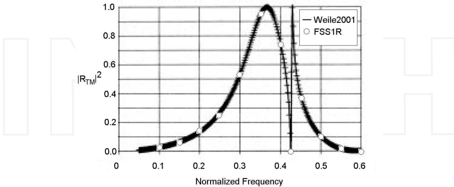
Fig. 8. Power reflection coefficient versus frequency (parallel polarization), normalization frequency was f_n = c/a = 16.842 GHz, \nu^i = 40 deg, \varphi^i = 0 deg
