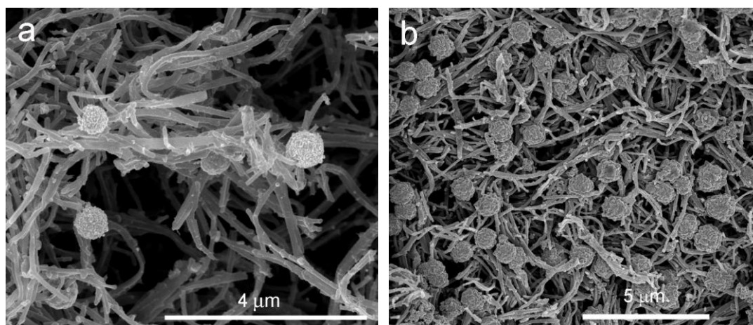
Figure 3. SEM images of after formation of Au clusters in presence of AA produced a) in one day (Au 2 @PNT) and b) in three days (Au 5 @PNT).
