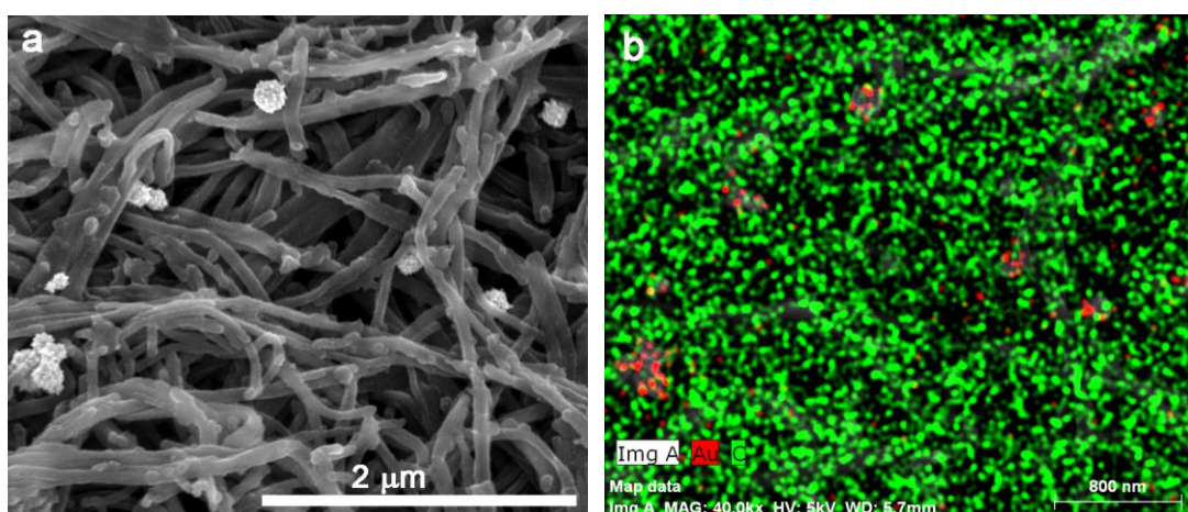
Figure 2. a) SEM image of Au 1 @PNT, b) SEM EDS analysis of Au 1 @PNT with Au visualized in red and C in green.
