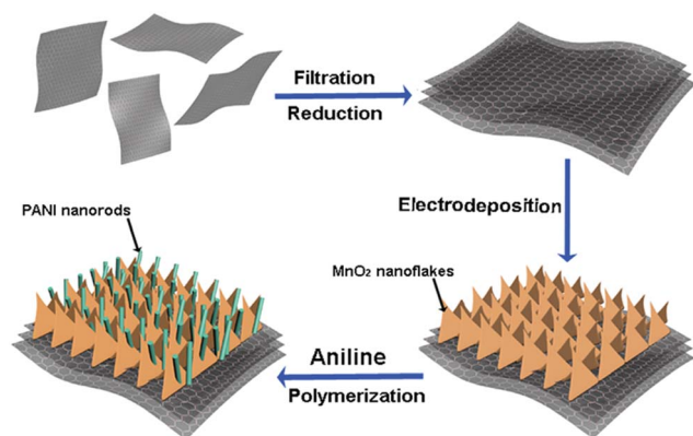
Fig. 1 Schematic illustration of the preparation process of the \text{RGO}/\text{MnO}_2/\text{PANI} nanocomposite.
