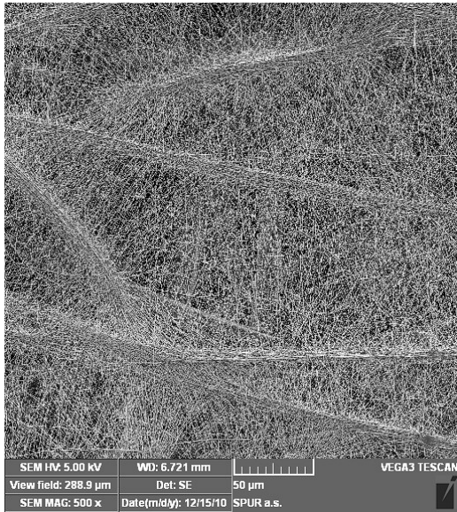
FIGURE 3. Accumulation of PU nanofibres around conductive microfibrils of a spunbond support, magnification 500×.
