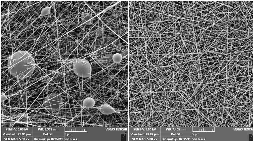
FIGURE 11. Nanostructure formed without any additives, magnification 5 000×.
