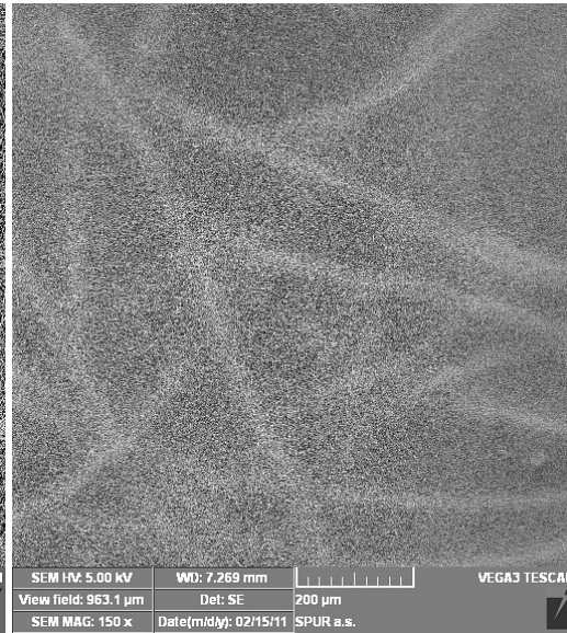
FIGURE 4. Homogenous lay-out of PU nanofibres around microfibrils of a spunbond support, magnification 150×.
