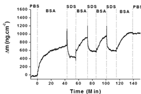
Figure 9. Mass variation versus time for a Ti quartz crystal. The experiment was performed at OCP and at 37^\circ\text{C} . The vertical dashed lines indicate switches between solutions: pure phosphate buffer saline (PBS, 0.01M), BSA (20 mg L -1 in PBS), SDS 0.09 M [89].
