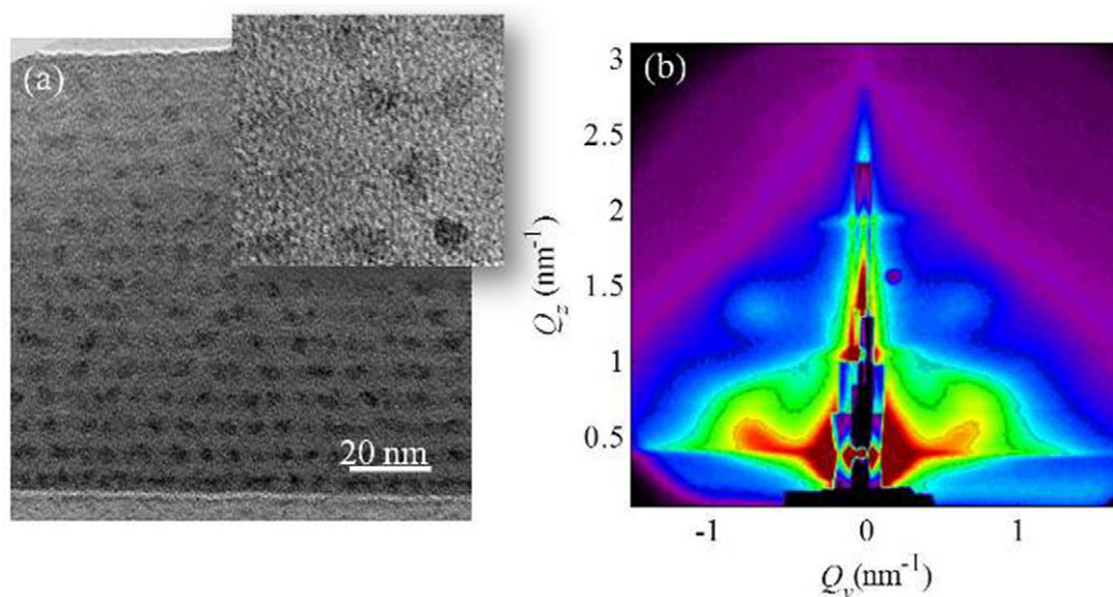
Figure 10. (a) TEM image of the Ge/Al 2 O 3 film and (b) the corresponding GISAXS map. The inset shows TEM image with better resolution.
