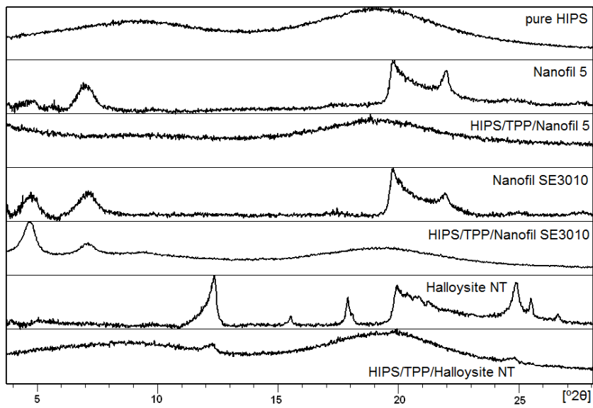
Figure 1. XRD spectra of pure nanofillers and composites with nanofillers.
