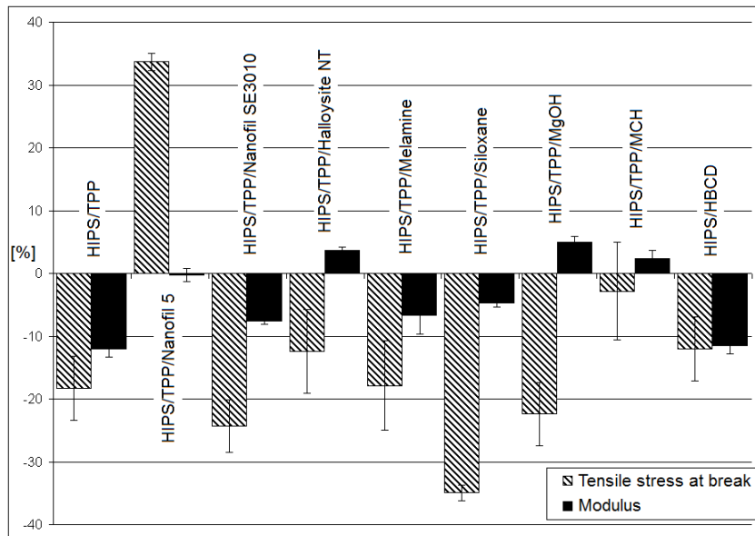
Figure 3. Comparison of tensile stress at break and modulus.
