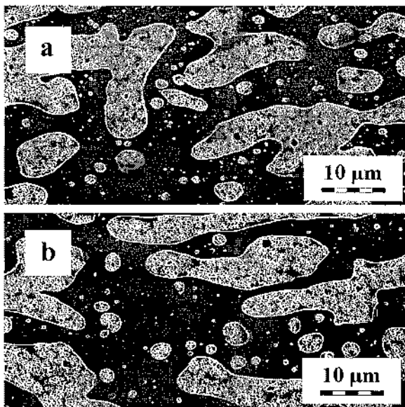
Figure 9 SEM of blend 64 taken from the middle of the CM sample (the cutting surfaces are perpendicular to each other).
