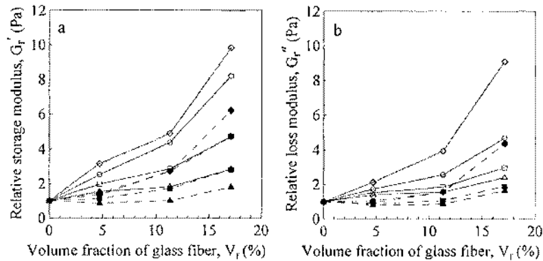
Figure 5 (a) Relative storage and (b) loss moduli as functions of glass fiber content for IM (open symbols) and CM (solid symbols) glass fiber filled blend 64 at various angular frequencies (rad/s): 0.1 ( \blacktriangleleft ); 1 (@); 10 (□); 100 (AA)- almost unaffected the sensitivity of the matrix,
