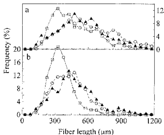
Figure 2 Fiber length distribution of glass fiber filled blend 64 (A CMP1, O CMP2, □ CMP3) prepared by (a) IM and (b) CM.
