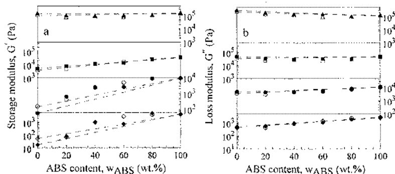
Figure 4 (a) Storage and (b) loss moduli as functions of ABS content for PC/ABS blends prepared by IM (open symbols) and CM (solid symbols) at various angular frequencies (rad/s): 0.1 ( \blacktriangle ); 1 ( \bullet ); 10 ( \square ); 100 ( \Delta ).
