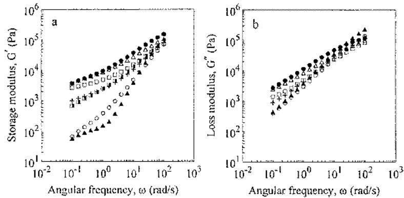
Figure 3 (a) Storage and (b) loss moduli as functions of angular frequency for pure materials ( \blacktriangle PC, \bullet ABS) and PC/ABS blends ( \circ blend 82, + blend 64, \square blend 46, \Delta blend 28) prepared by IM and blend 46 ( \square ) by CM.
