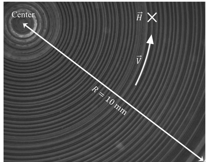
Figure 2. Concentric layers formed in a plate-plate configuration when a magnetic field is applied in the velocity gradient direction. Particle concentration \phi = 10 vol%. External magnetic field strength H = 10.81 kA m ^{-1} . Rim shear rate \dot{\gamma}_R = 300 s ^{-1} .
