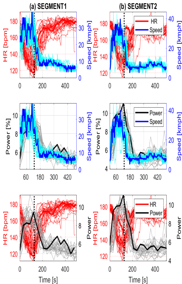
FIGURE 6. Comparison of the heart rate vs. speed, the relative mean power of the accelerometric signal in the frequency range (30, 40) Hz vs. speed, and the heart rate vs. the relative mean power in the frequency range (30, 40) Hz for 26 cycling experiments and the dash line separating downcycling and upcycling specified by the cadence sensor.
