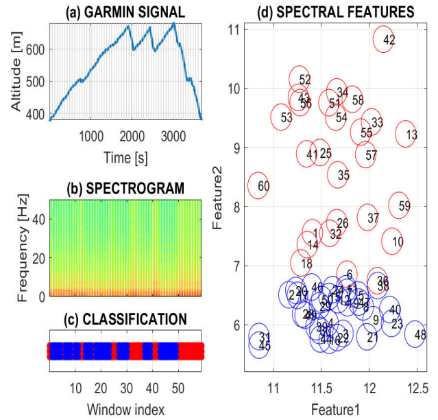
FIGURE 3. Feature extraction for (a) the cycling route recorded by the GNSS signal and divided into segments with a selected length of 60 s, (b) spectrogram of the accelerometric signal, (c,d) features specified into two selected spectral regions, and clustering results from the unsupervised Kohonen learning process.
