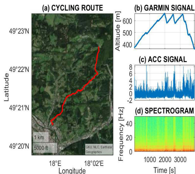
FIGURE 1. The area of cycling experiments presenting (a) the cycling route in the geographical environment, (b) the altitude GPS signal recorded by the Garmin system, (c) the accelerometric (ACC) signal recorded by the mobile sensor, and (d) spectrogram of a selected experiment.
