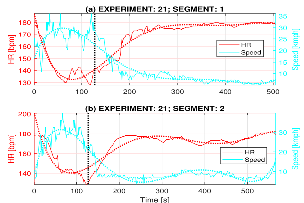
FIGURE 5. The polynomial approximation of the heart rate and the speed during a selected cycling experiment in (a) segment 1 and (b) segment 2 with the dash line separating downcycling and upcycling specified by the cadence sensor.
