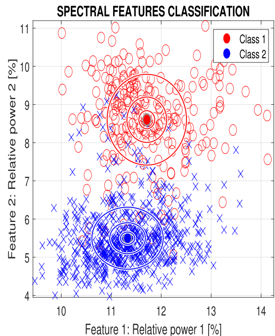
FIGURE 7. Classification of spectrogram features related to accelerometric data of all experiments using the relative mean power in selected frequency ranges (F1 : (10, 15) Hz and F2 : (30, 40) Hz) presenting segments belonging to class 1 (downhill cycling) and class 2 (uphill cycling) using the two layer neural network with centers of gravity of individual classes and c-multiples of standard deviations for c = 0.2, 0.5, 1.
