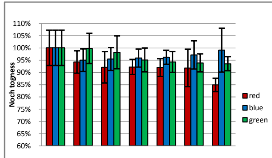
Fig. 10 Proportional graph of notch toughness
