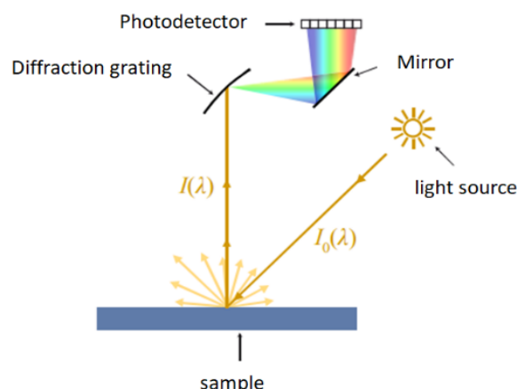
Fig. 3 Color sensing
