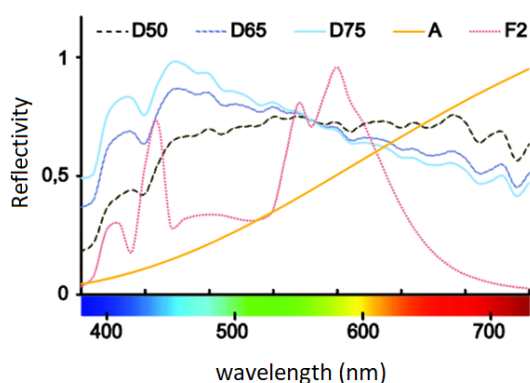
Fig. 4 . Reflective spectrum
