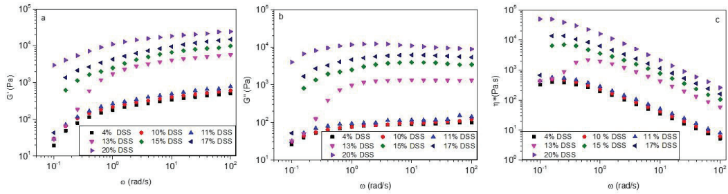
FIGURE 3. Frequency sweep for guar gum gel with different amount of DSS: a) storage modulus, b) loss modulus, and c) complex viscosity.
